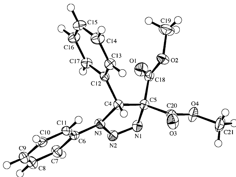
Fig. 3. ORTEP Plot [25] of the molecular structure of 10 (50% probability ellipsoids, arbitrary numbering of atoms)
