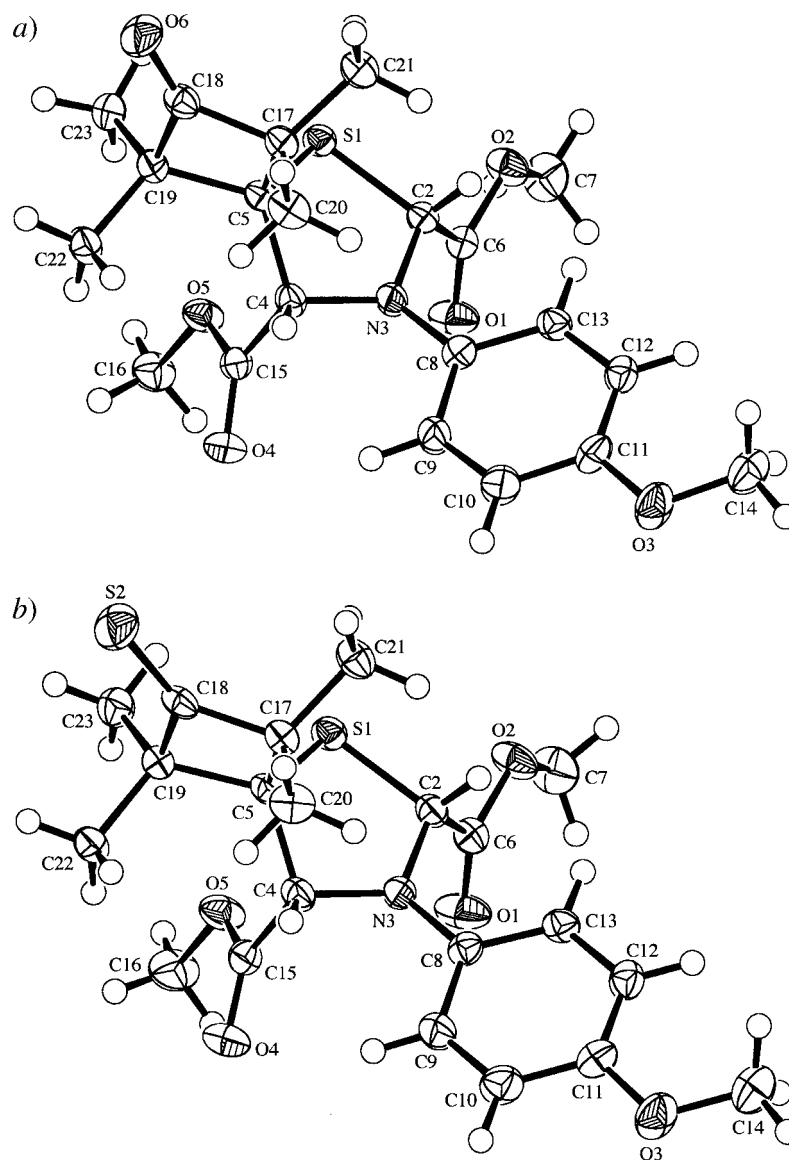
Fig. 2. ORTEP Plot [25] of the molecular structure of a) cis- 8a and b) cis- 8b (50% probability ellipsoids, arbitrary numbering of atoms)
