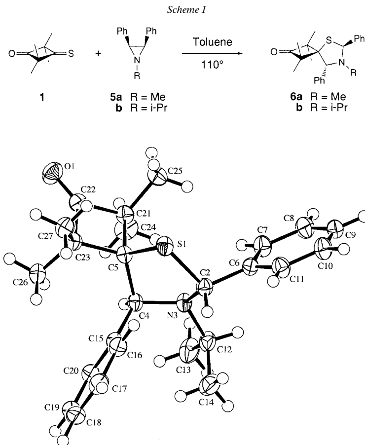
Fig. 1. ORTEP Plot [25] of the molecular structure of 6b (50% probability ellipsoids, arbitrary numbering of atoms)
