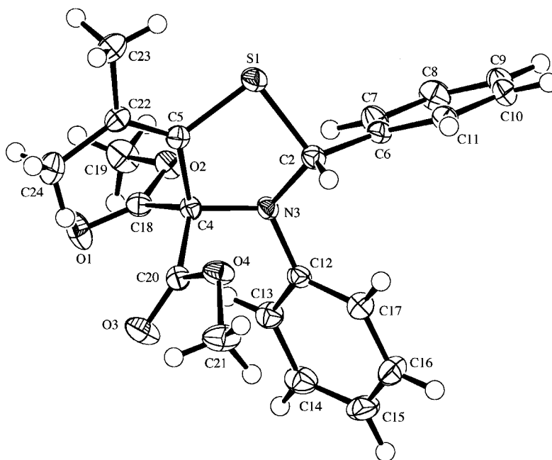
Fig. 4. ORTEP Plot [25] of the molecular structure of 16 (50% probability ellipsoids, arbitrary numbering of atoms)
